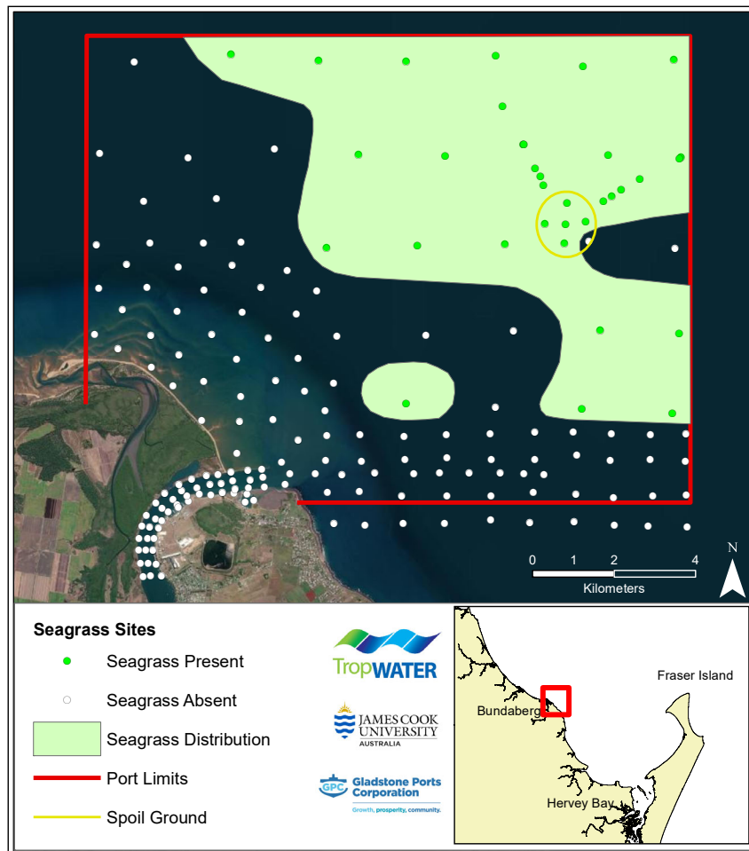
Figure 4. Seagrass presence/absence at sites surveyed and seagrass distribution within Port of Bundaberg in 2020.
